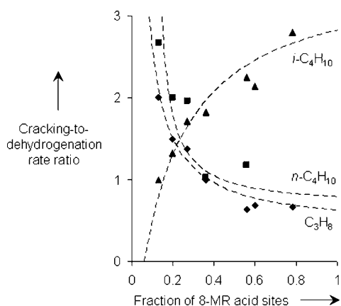
Figure 2. Cracking-to-dehydrogenation rate ratios (748 K) for propane (♦), n -butane (■) and isobutane (▲) on H-MOR catalysts with different fractions of Brønsted acid sites within 8-MR side pockets; rate ratios predicted using regressed rate constants are given by the dashed curves.
