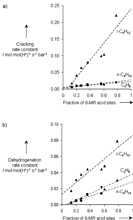
Figure 1. Dependence of rate constants (748 K) for monomolecular a) cracking and b) dehydrogenation of propane ( \times 10 ; ♦), n -butane (■), and isobutane (▲) on the fraction of 8-MR acid sites in H-MOR catalysts.
